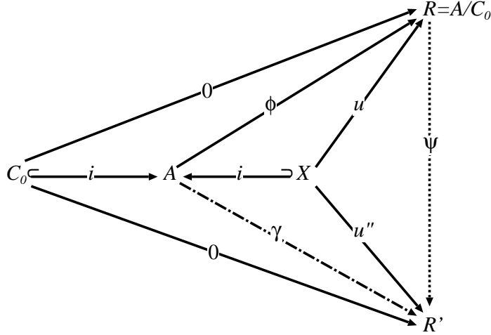
Figure 1: A commuting diagram illustrating the proof of the universal property in Theorem 1. Here i represents an inclusion map (regard \mathcal{X} as a subset of \mathcal{A} in the obvious way) and 0 represents a zero homomorphism.
