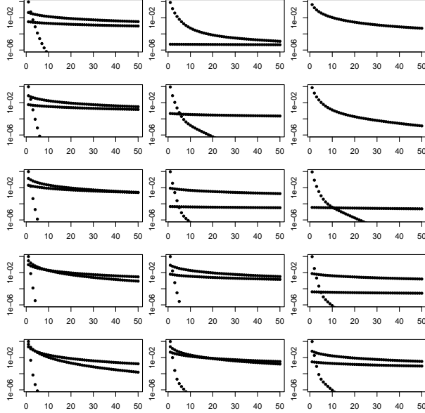
FIGURE 1. Probabilities of numbers of rejections on a log scale. Values of \phi are, from top to bottom, 0.8, 0.9, 0.95, 0.98 and 0.99. Values of the coefficient of variation of volatility are, from left to right, 0.25, 0.75 and 2.5.
